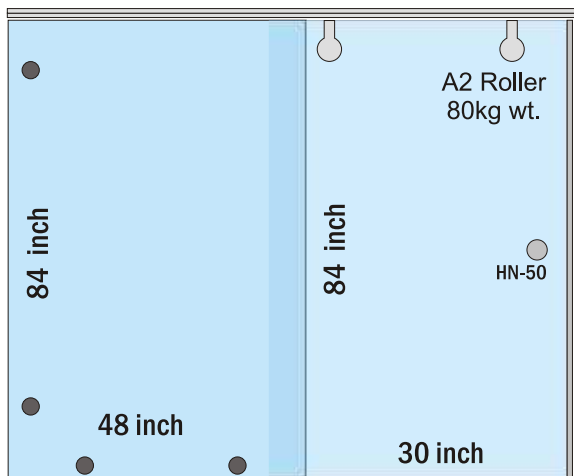
Sliding Door -8mm / 10mm (6ft rod)
