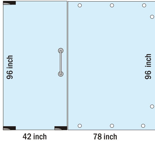
Glass Door -10mm / 12mm (10 x 8 ft)
