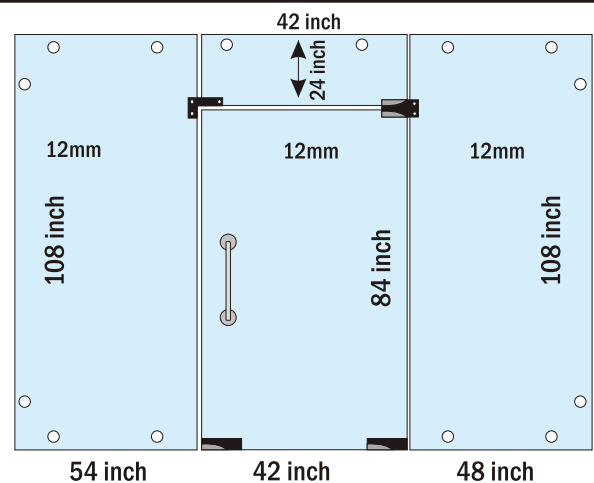
Glass Door -10mm / 12mm (12x9 ft)
