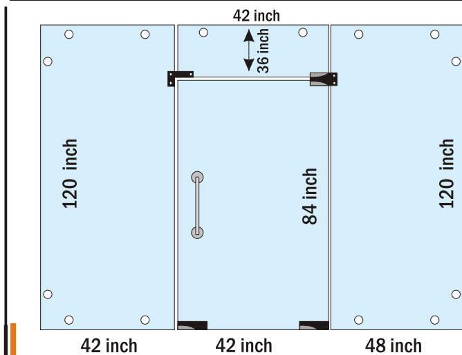
Glass Door -10mm / 12mm (11x10 ft)
