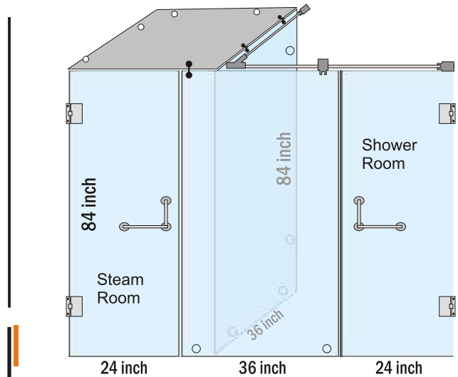
Glass Door -8mm / 10mm (7x7x3/4 ft) FIX PRICE : 31,350/32,950 / Inside 4ft- 31,780/33,400
