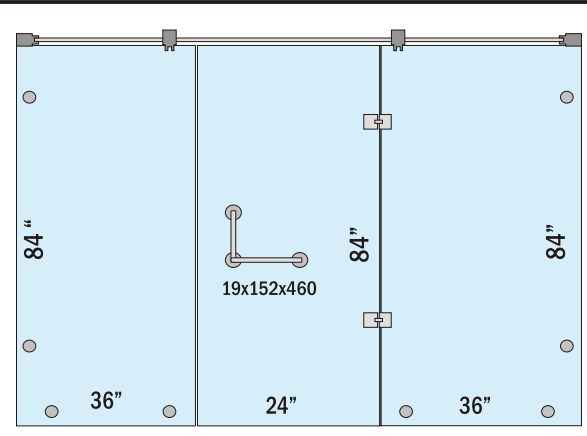
Wall-wall--180° hinge- 7/8 ft (Heavy Rod)
