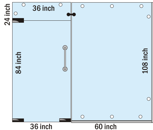
Glass Door -10mm / 12mm (8 x 9/10 ft)
