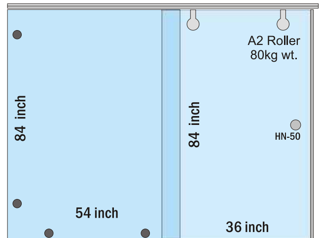
Sliding Door -8mm / 10mm (7 ft rod)
