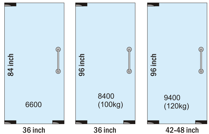
Only Glass Door -12mm
