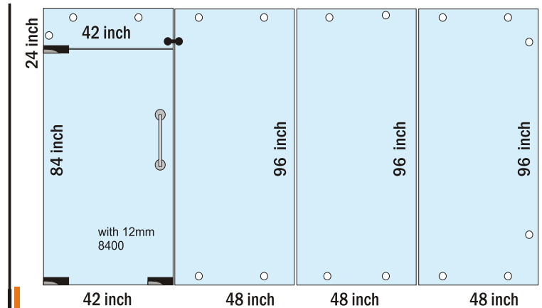
Glass Door -10mm / 12mm (16x9 ft)
