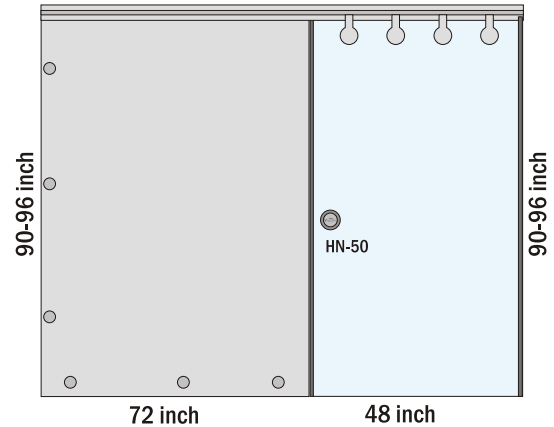
Sliding Door -8mm / 10mm (9-10 ft rod)
