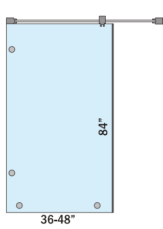
Fix Partition, 3-4 ft
