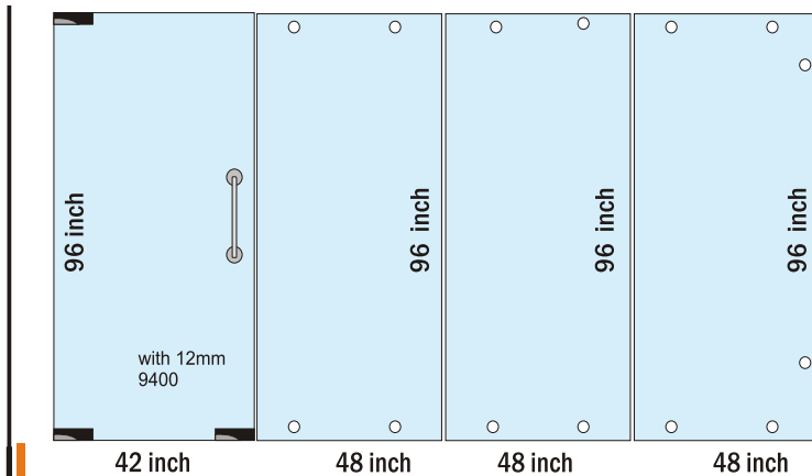
Glass Door -10mm / 12mm (16x8 ft)
