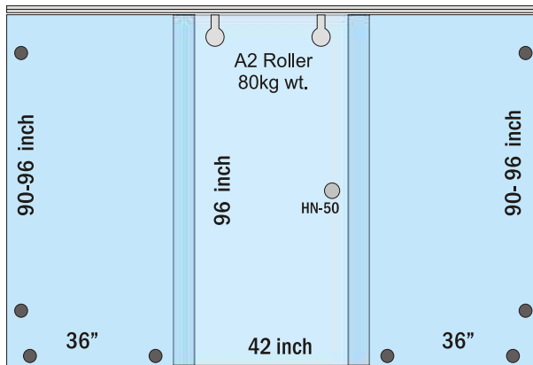
Sliding Door -8mm / 10mm (8--9 ft rod)
