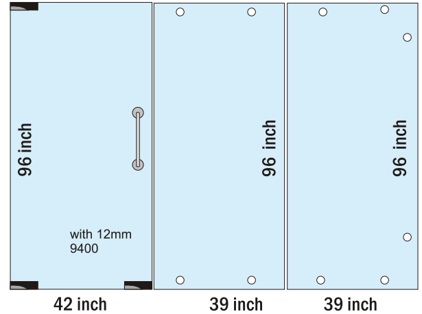
Glass Door -10mm / 12mm (11x8 ft)
