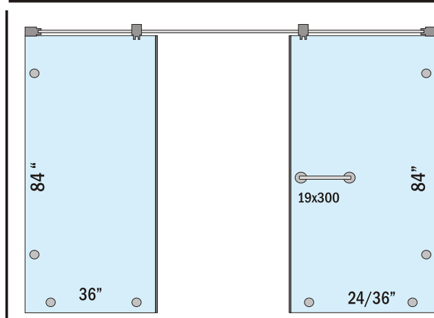
Wall-wall shower only 2 fix - 7/8 ft
