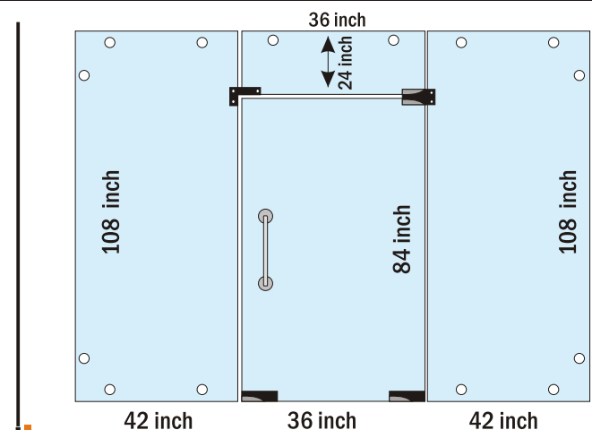
Glass Door -10mm / 12mm (10x9/8 ft)
