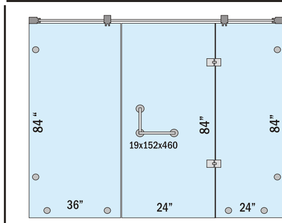
Wall-wall--180° hinge- 6 / 7 ft
