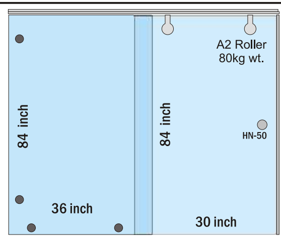
Sliding Door -8mm / 10mm (5ft rod) 1 fix 1 Door, FIX PRICE : 15,950.00 / 16,620.00
