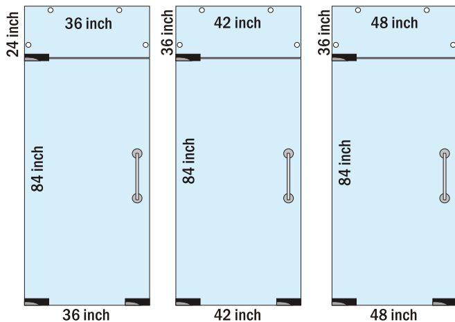
Only Glass Door -10mm / 12mm
