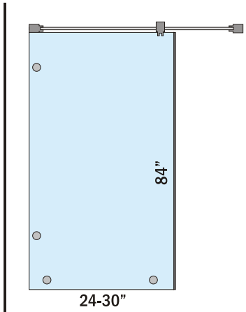
Fix Partition, 2-2.6 ft
