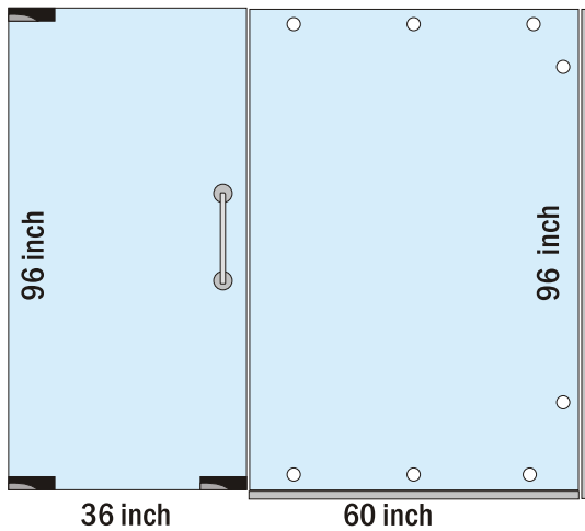
Booth Glass Door -10mm / 12mm (8 x 8 ft)
