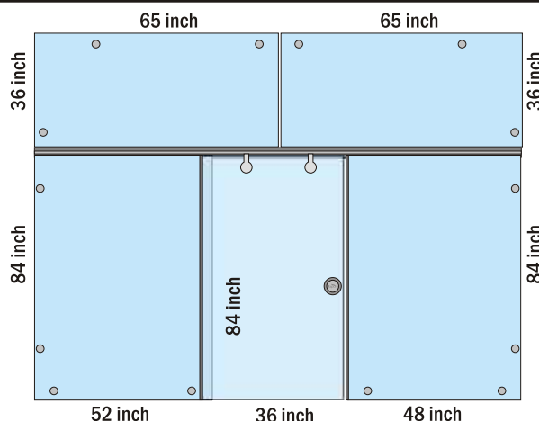
Balcony partition -8 / 10mm (10-11 ft rod)
